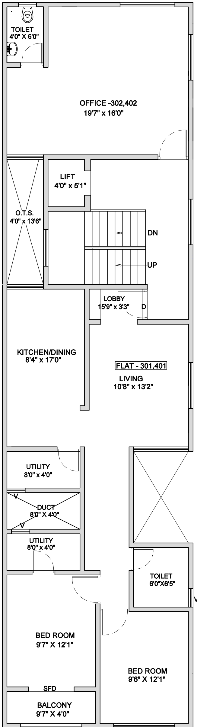
TYPICAL THIRD & FOURTH FLOOR PLAN
